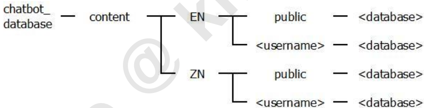
Figure 4-11 Directory Structure
