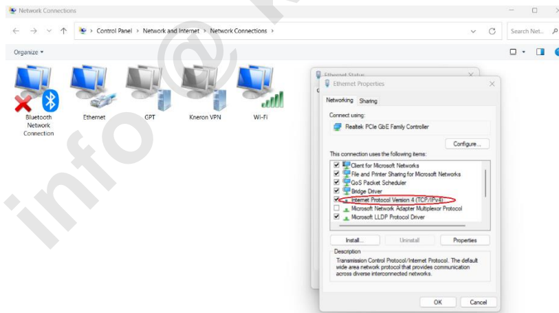
Figure 4-6 Ethernet Properties
