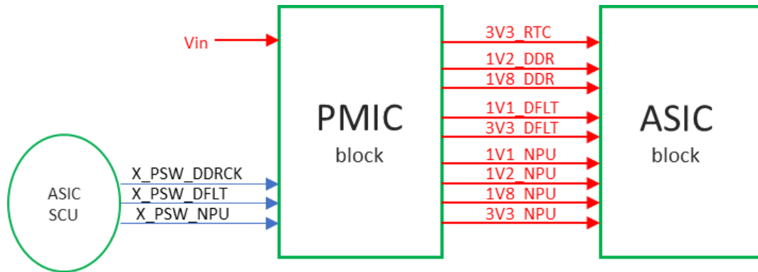
Figure 2 – Power topology
