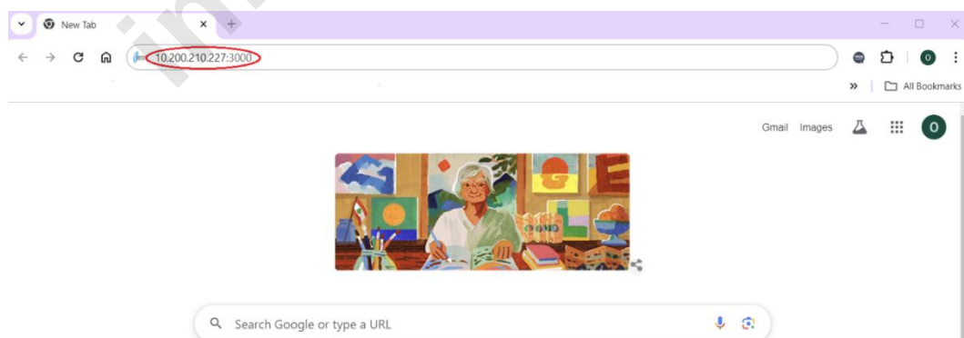
Figure 2-3 Browser Access
