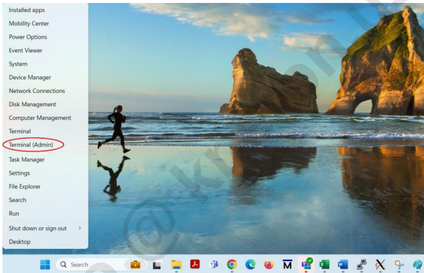
Figure 3-3 Window PowerShell
