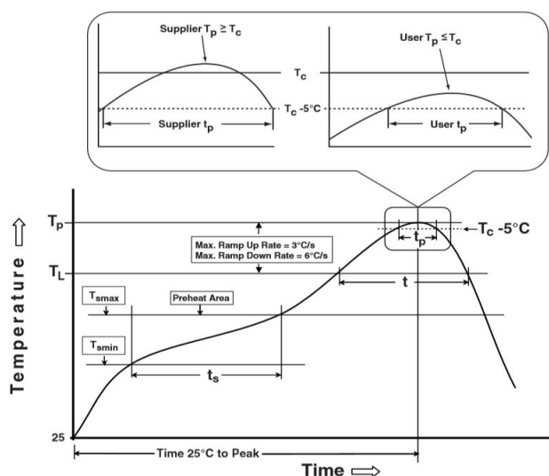
Reflow profile
